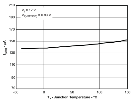
Figure 15. Shutdown Supply Current vs Junction Temperature
