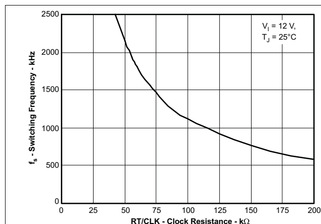
Figure 31. High-Range RT
