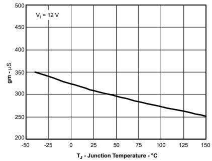
Figure 8. EA Transconductance vs Junction Temperature
