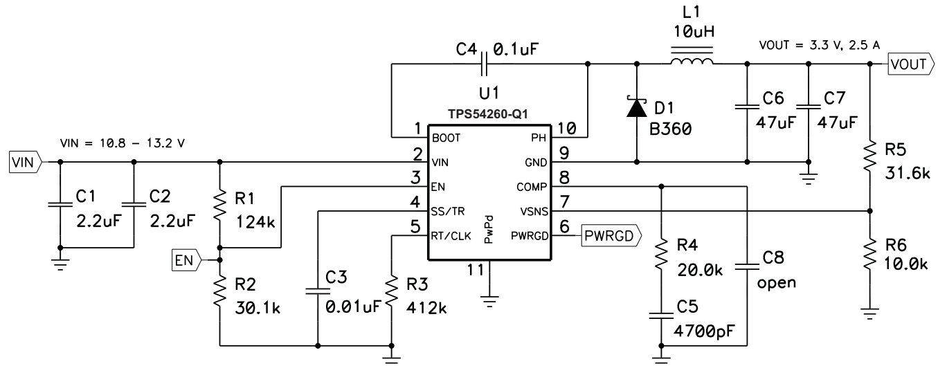
Figure 50. 3.3-V Output TPS54260-Q1 Design Example
